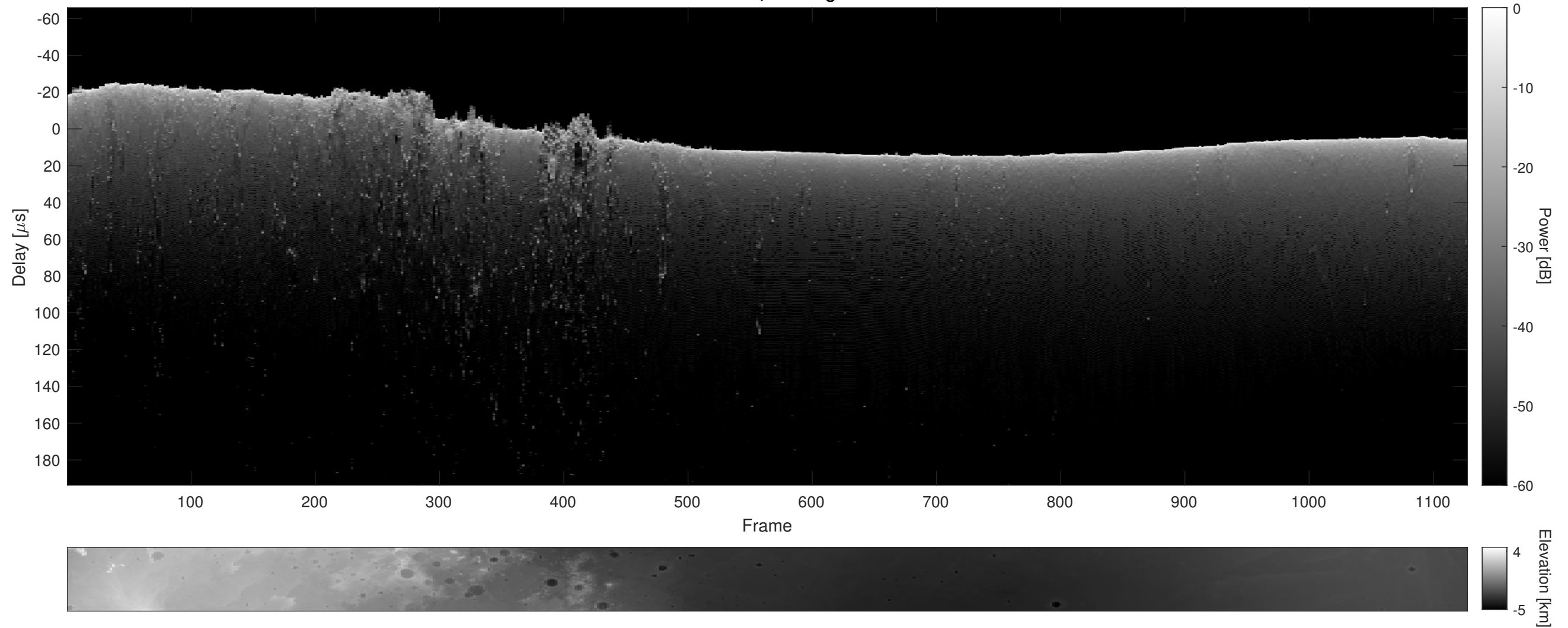
Orbit 14359, Cluttergram
