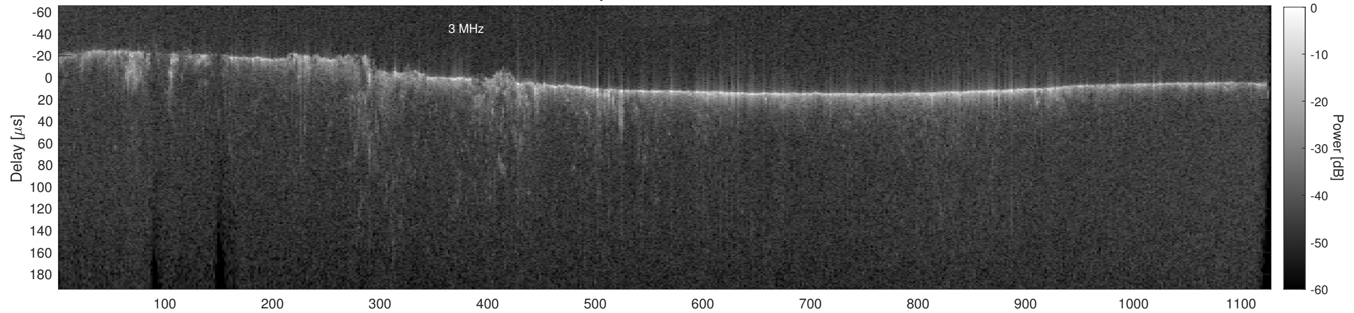
Orbit 14359, Cluttergram
