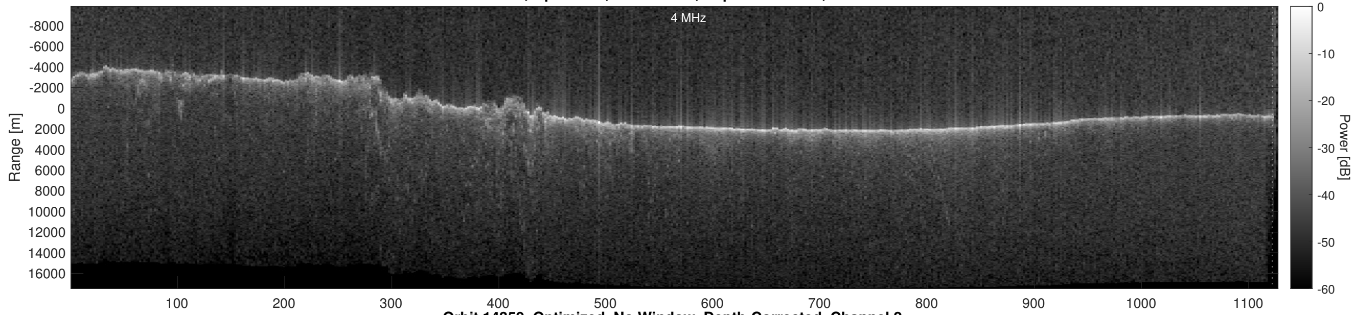
Orbit 14359, Optimized, No Window, Depth-Corrected, Channel 2
