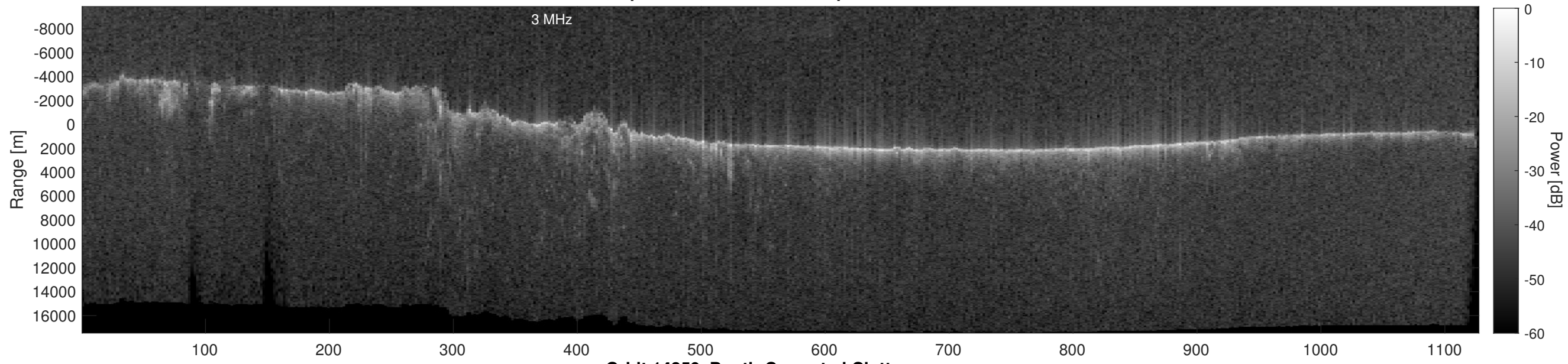
Orbit 14359, Depth-Corrected Cluttergram
