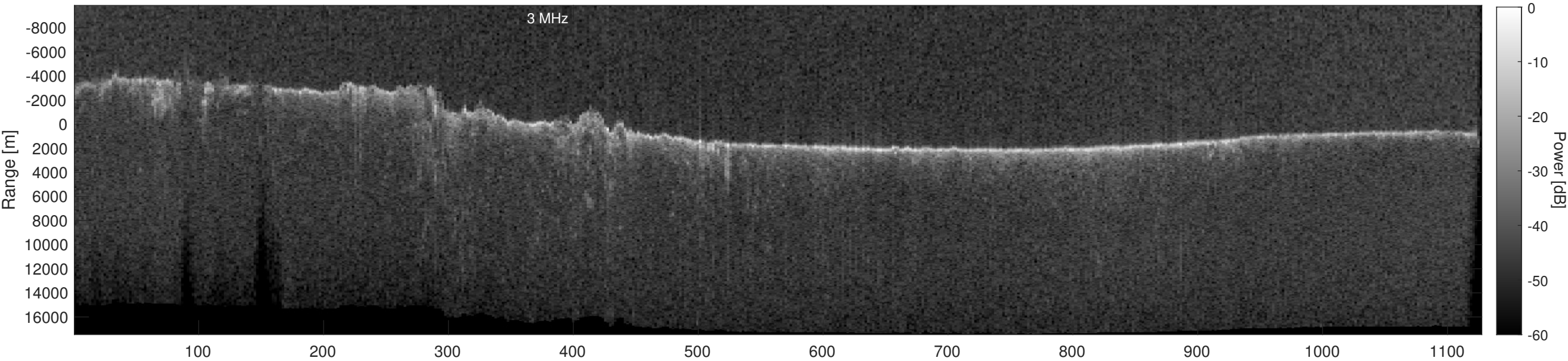
Orbit 14359, Depth-Corrected Cluttergram
