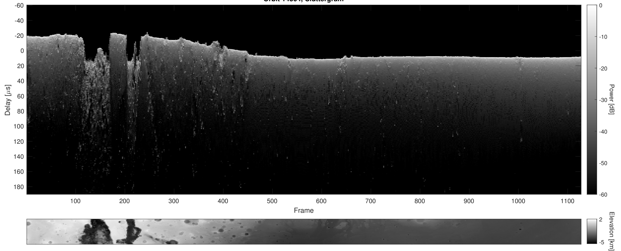
Orbit 14364, Cluttergram
