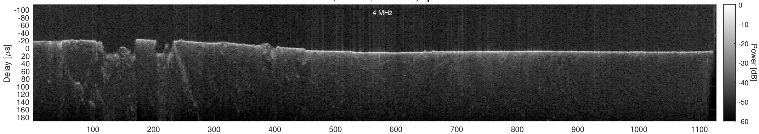
Orbit 14364, Cluttergram
