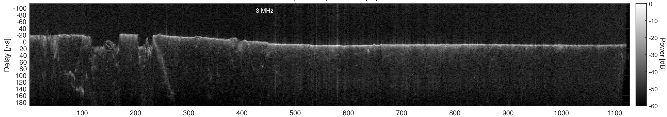
Orbit 14364, Cluttergram
