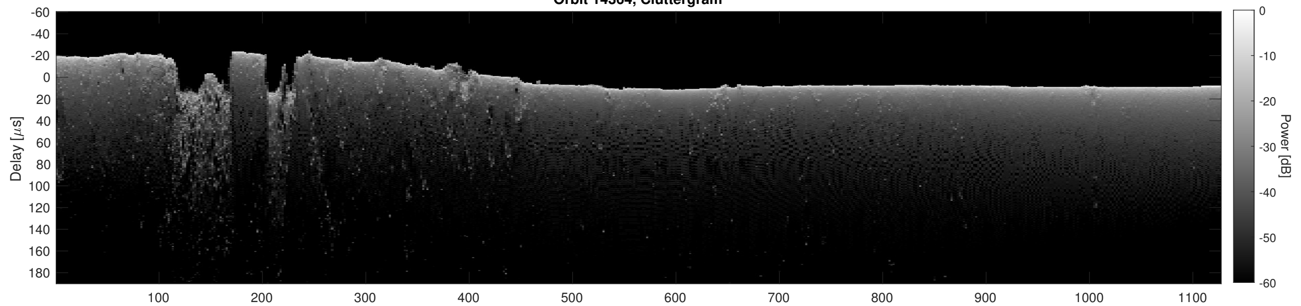
Orbit 14364, Cluttergram
