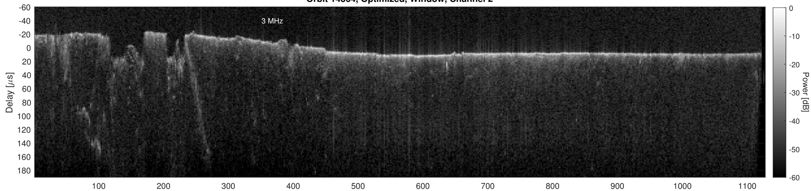
Orbit 14364, Cluttergram
