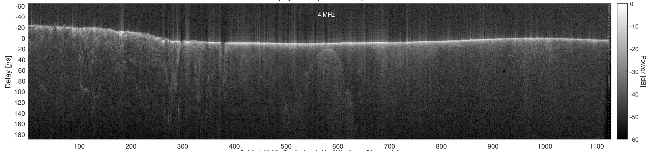
Orbit 14365, Optimized, No Window, Channel 2
