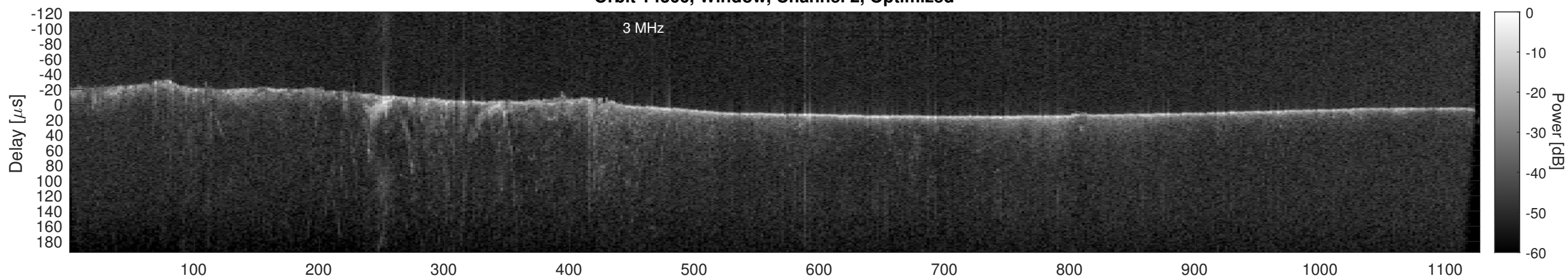
Orbit 14366, Cluttergram
