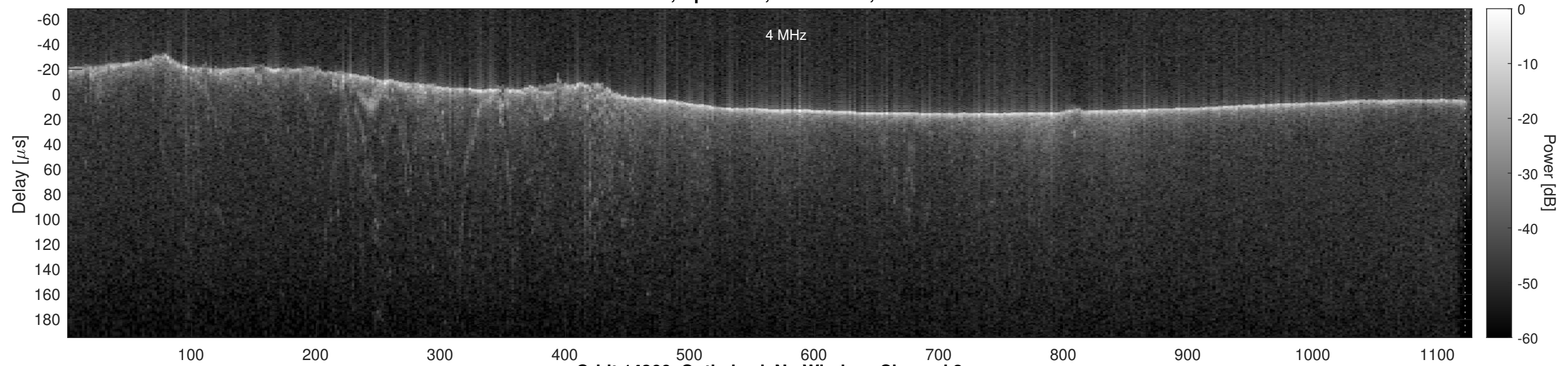
Orbit 14366, Optimized, No Window, Channel 2
