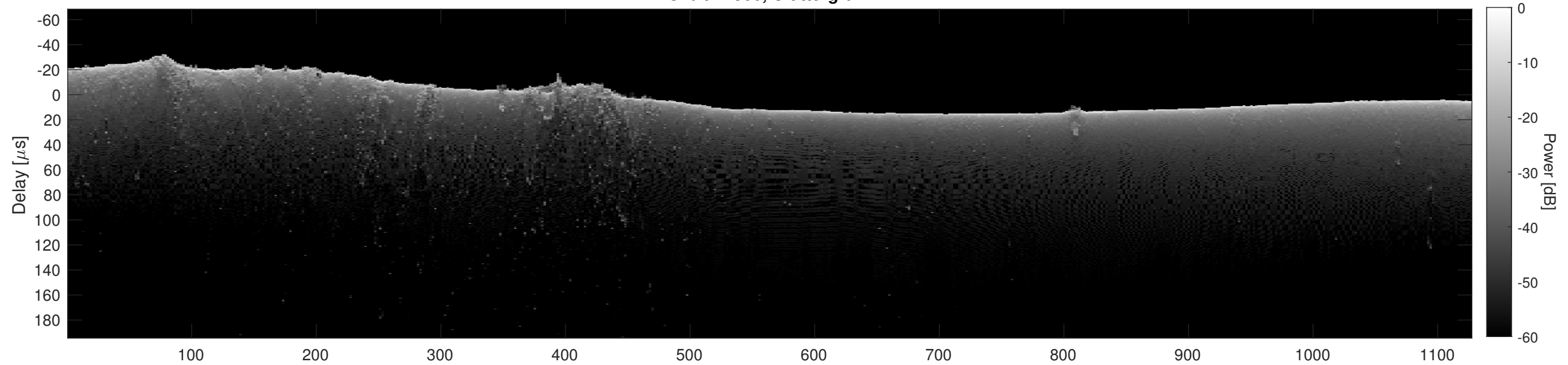
Orbit 14366, Cluttergram
