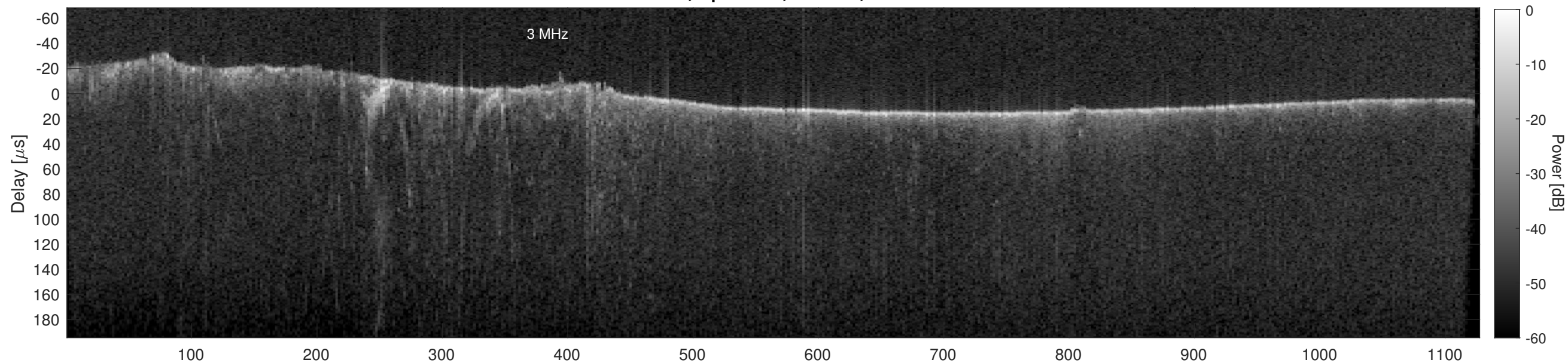
Orbit 14366, Cluttergram
