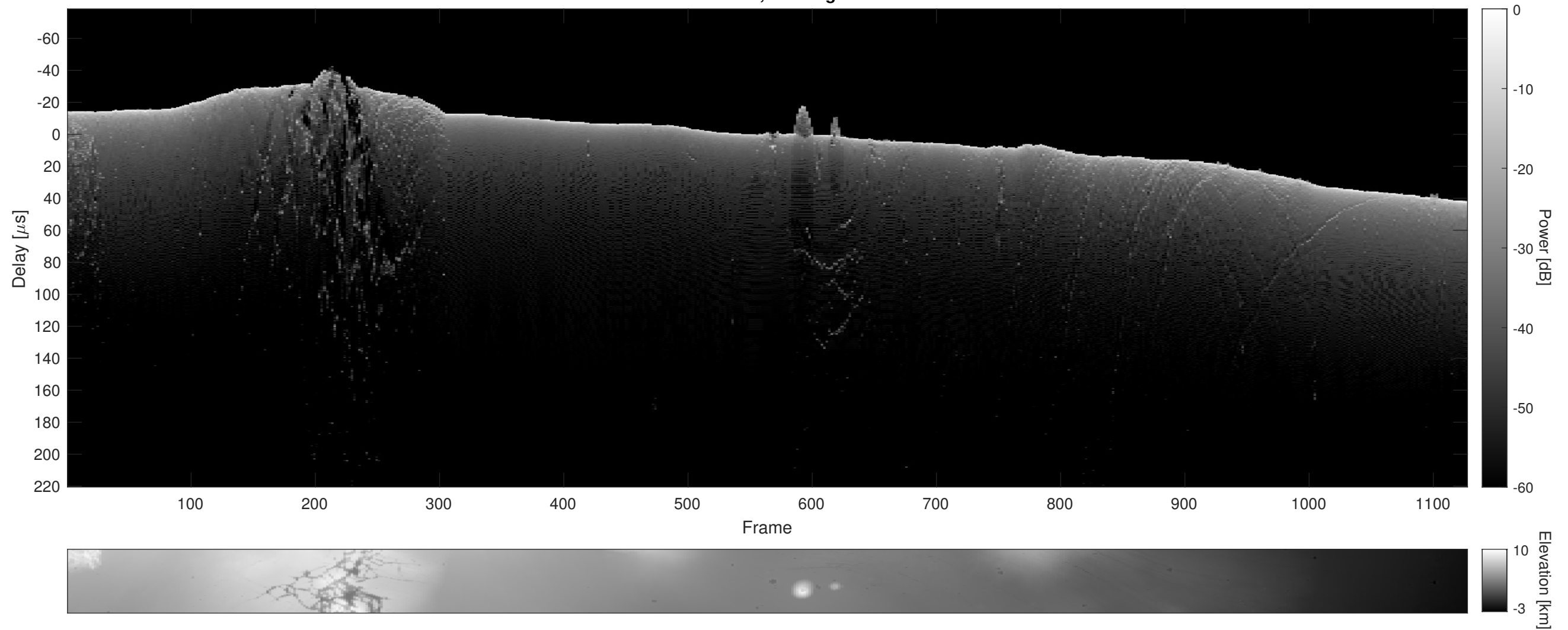
Orbit 14368, Cluttergram
