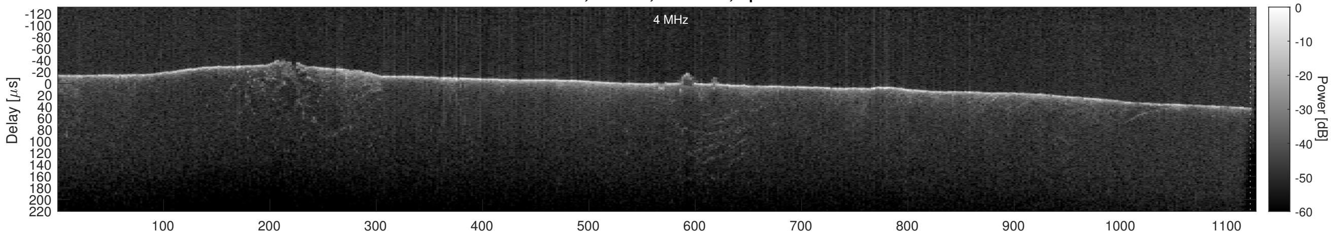
Orbit 14368, Cluttergram
