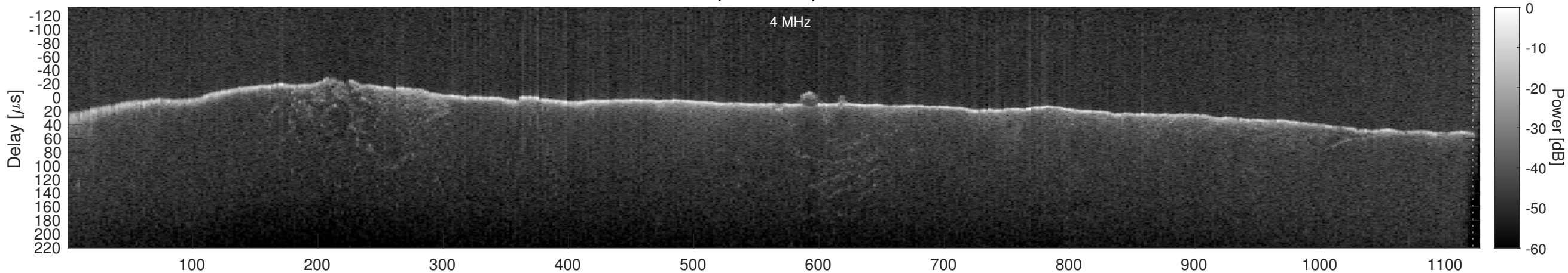
Orbit 14368, Window, Channel 1, Chapman
