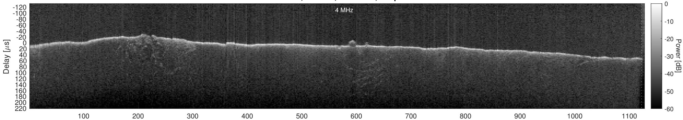
Orbit 14368, Window, Channel 1, Optimized
