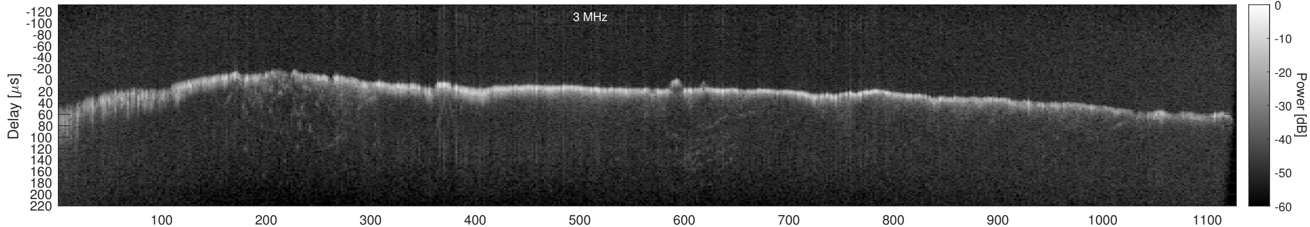
Orbit 14368, Window, Channel 2, Chapman
