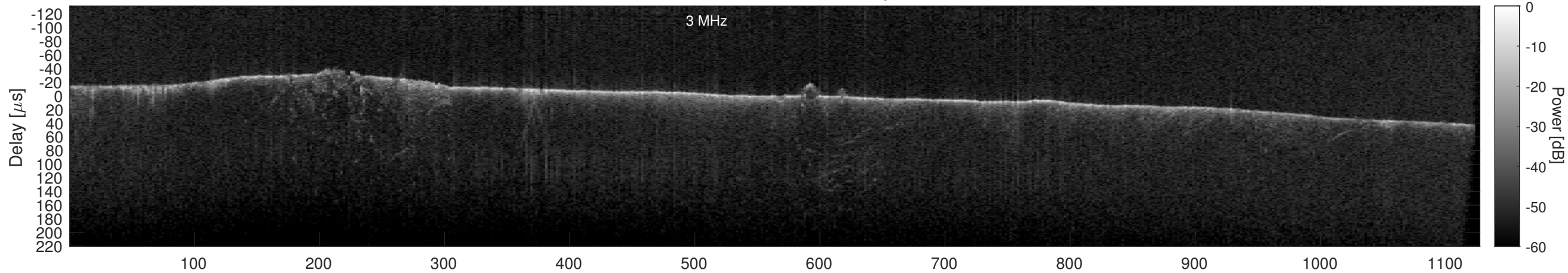
Orbit 14368, Cluttergram
