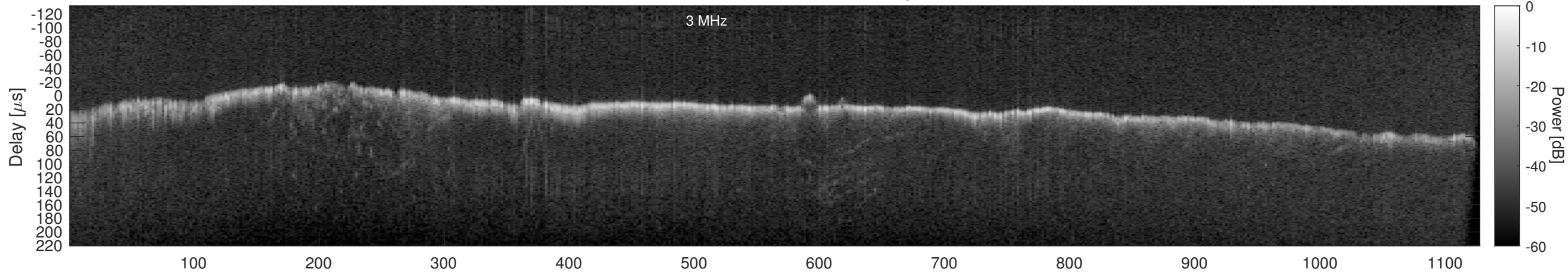
Orbit 14368, Window, Channel 2, Optimized
