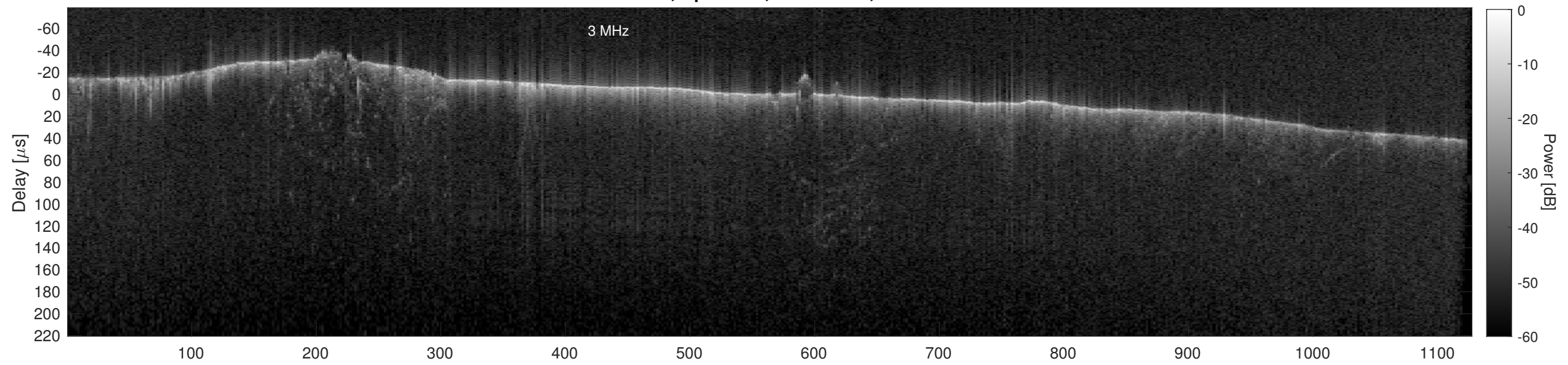
Orbit 14368, Cluttergram
