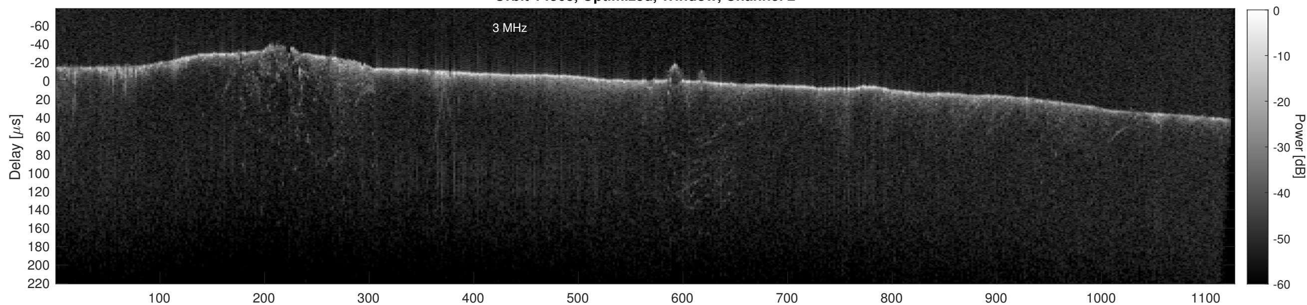
Orbit 14368, Cluttergram
