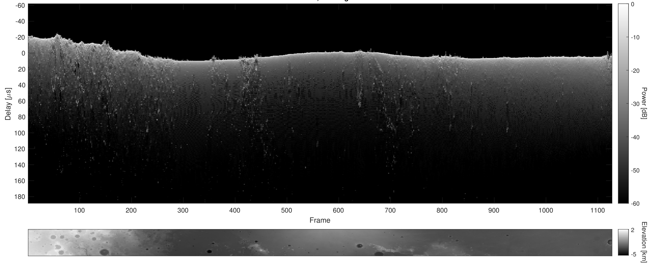
Orbit 14369, Cluttergram
