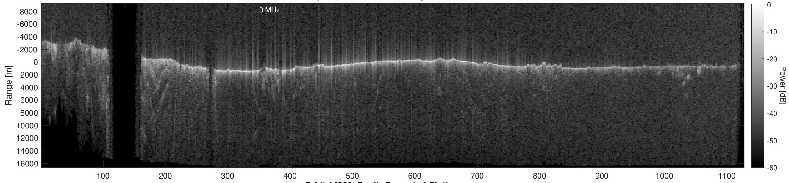
Orbit 14369, Depth-Corrected Cluttergram
