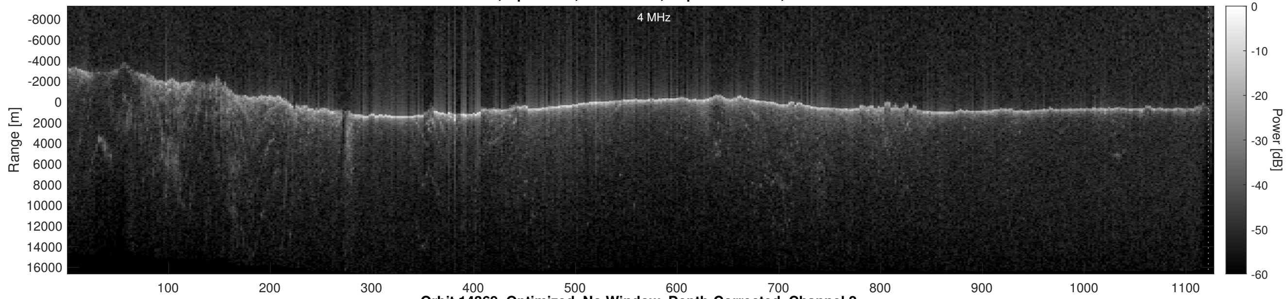
Orbit 14369, Optimized, No Window, Depth-Corrected, Channel 2
