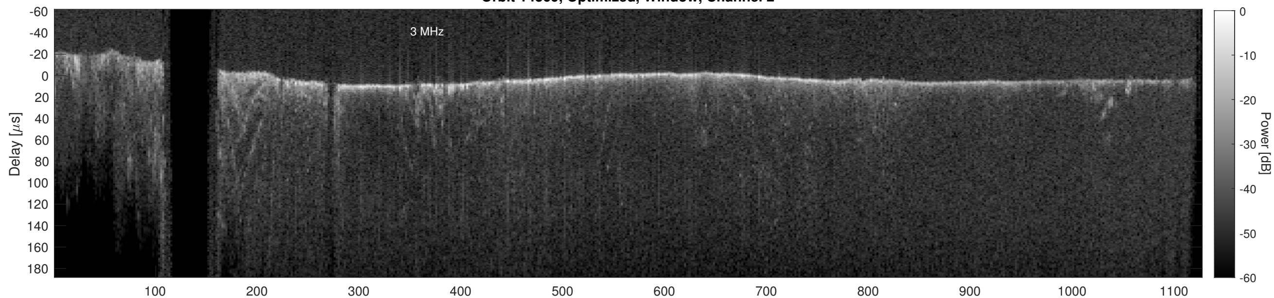
Orbit 14369, Cluttergram
