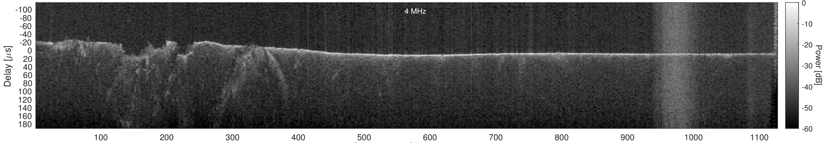
Orbit 14371, Cluttergram
