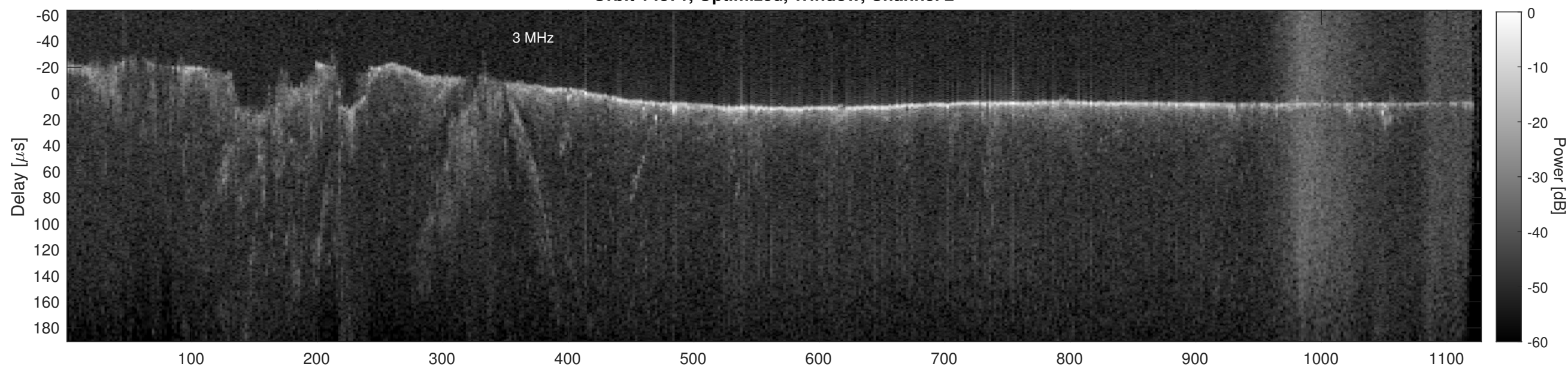
Orbit 14371, Cluttergram
