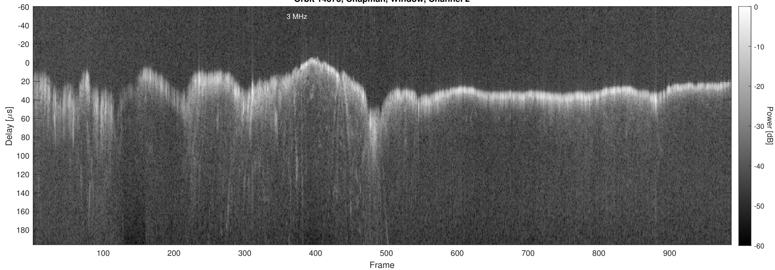
Orbit 14373, Chapman, Window, Channel 2
