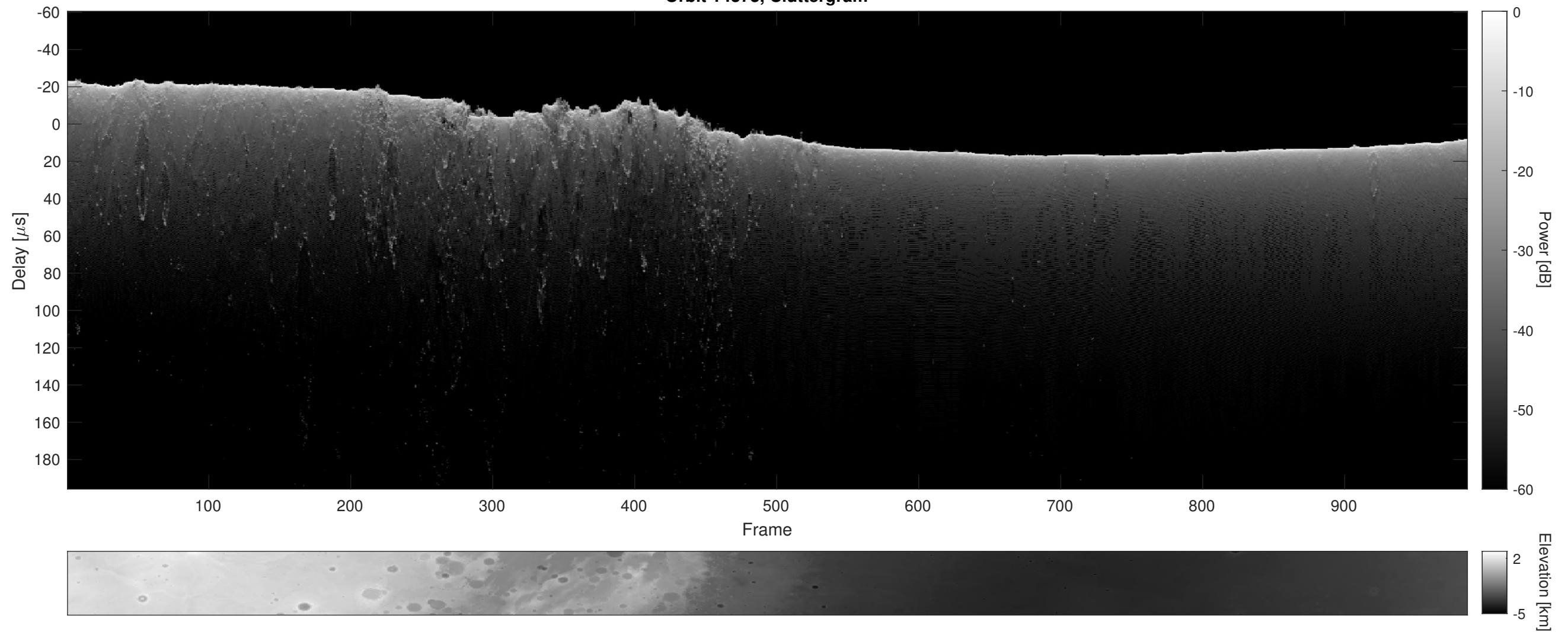
Orbit 14373, Cluttergram
