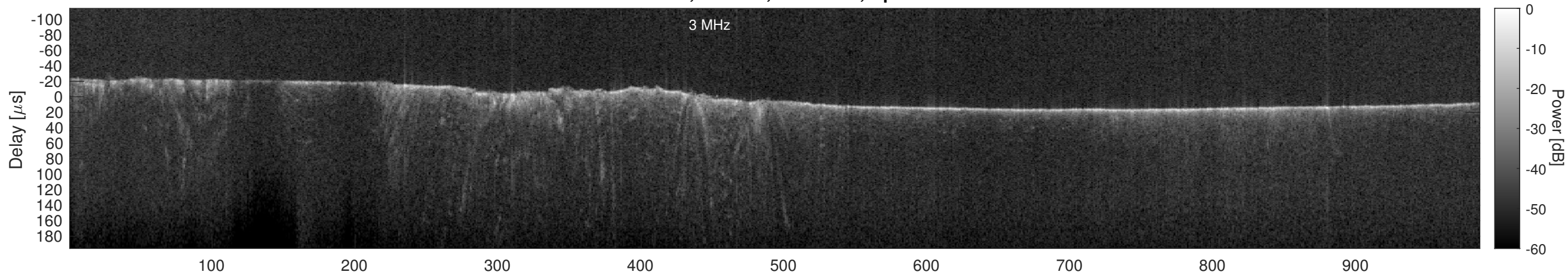
Orbit 14373, Cluttergram
