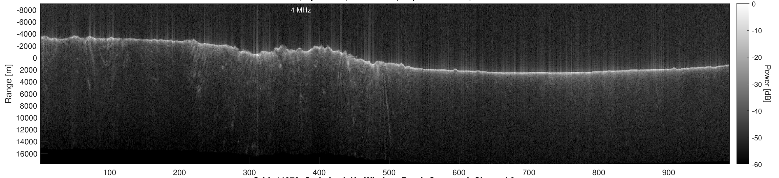
Orbit 14373, Optimized, No Window, Depth-Corrected, Channel 2
