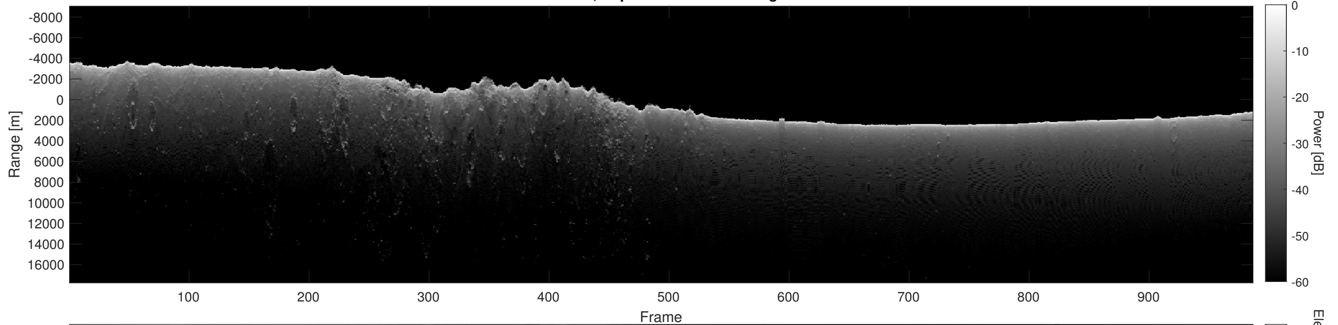
Orbit 14373, Depth-Corrected Cluttergram
