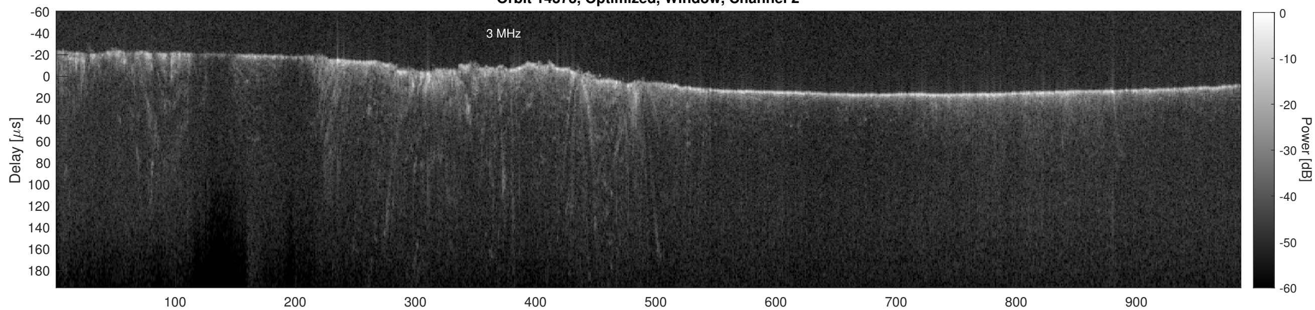
Orbit 14373, Cluttergram
