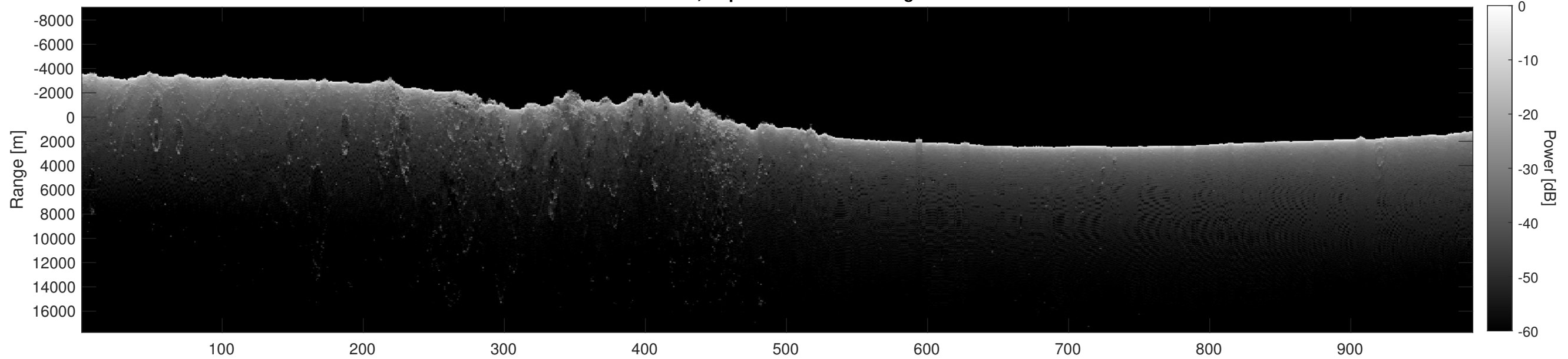
Orbit 14373, Depth-Corrected Cluttergram
