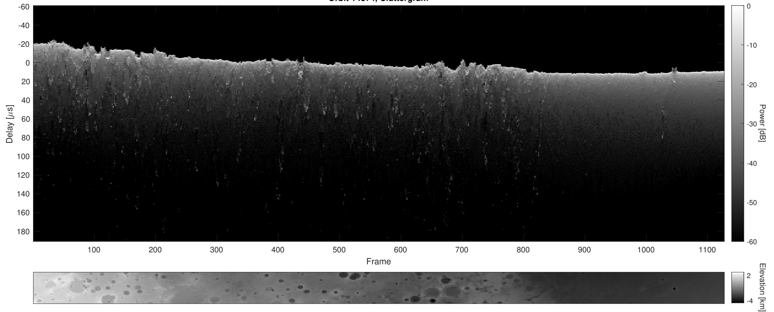
Orbit 14374, Cluttergram
