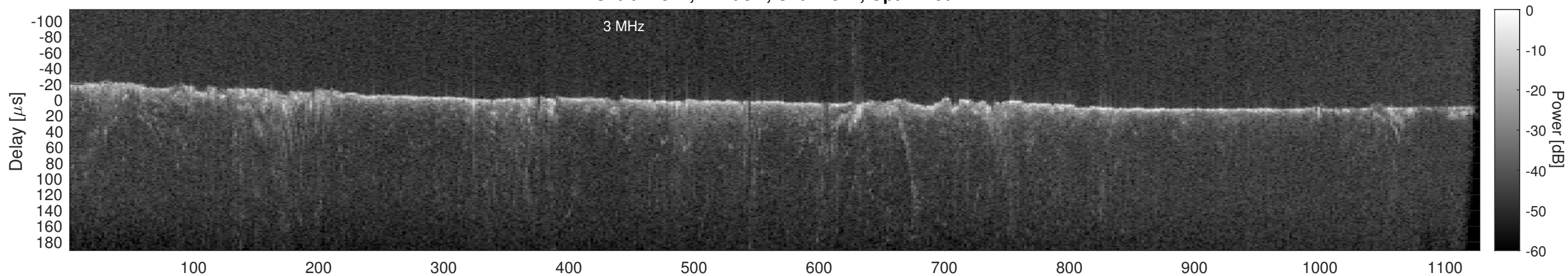
Orbit 14374, Cluttergram
