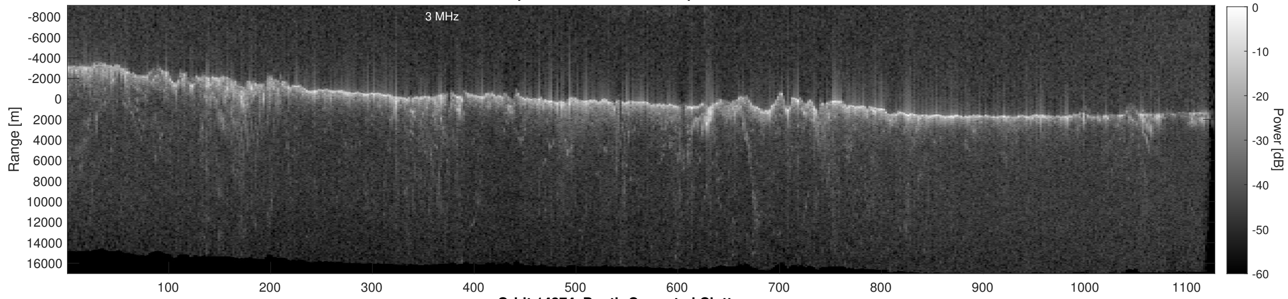
Orbit 14374, Depth-Corrected Cluttergram
