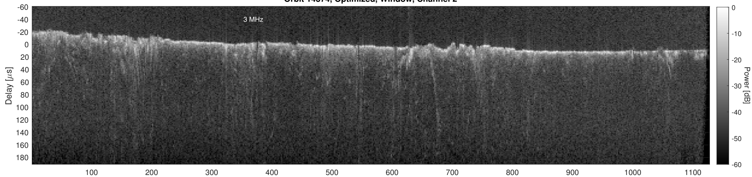
Orbit 14374, Cluttergram
