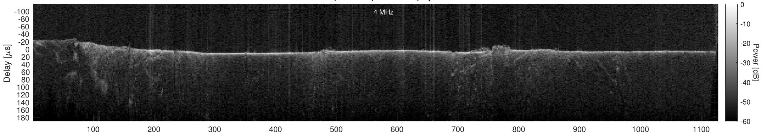
Orbit 14376, Cluttergram
