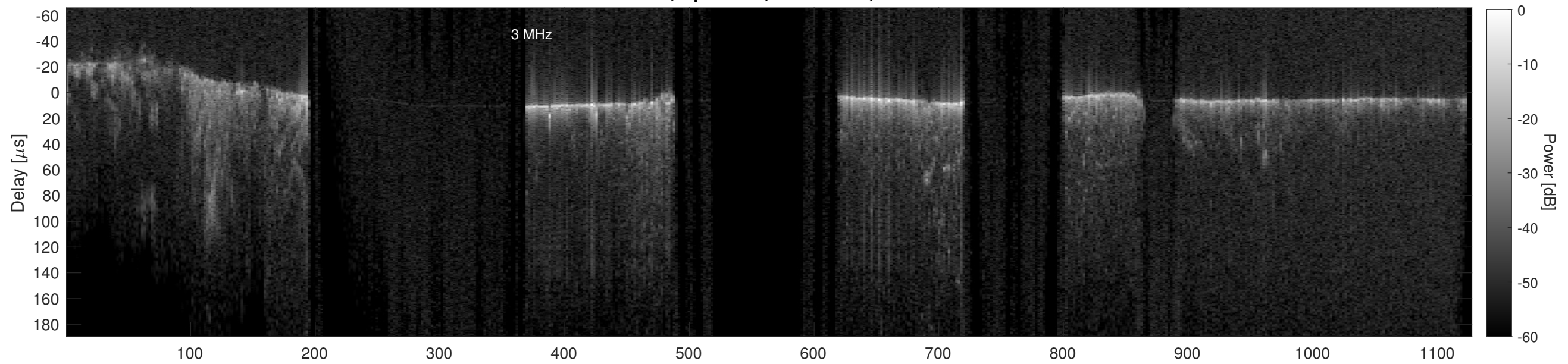
Orbit 14376, Cluttergram
