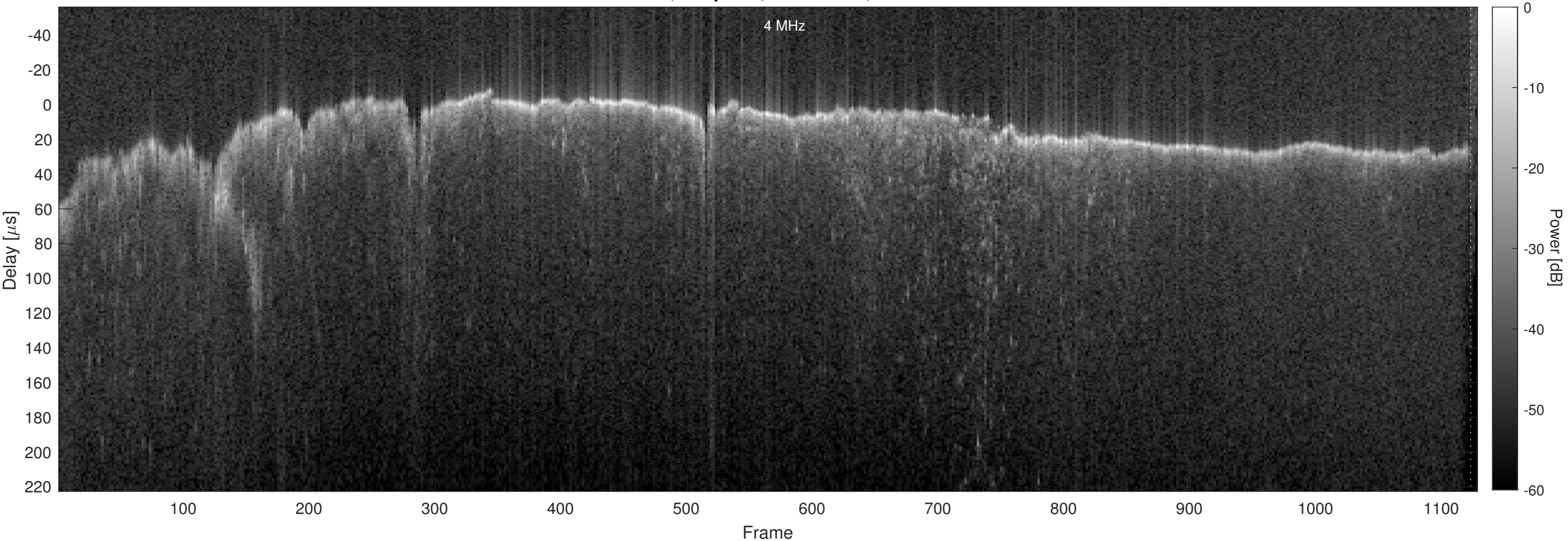
Orbit 14377, Chapman, No Window, Channel 2
