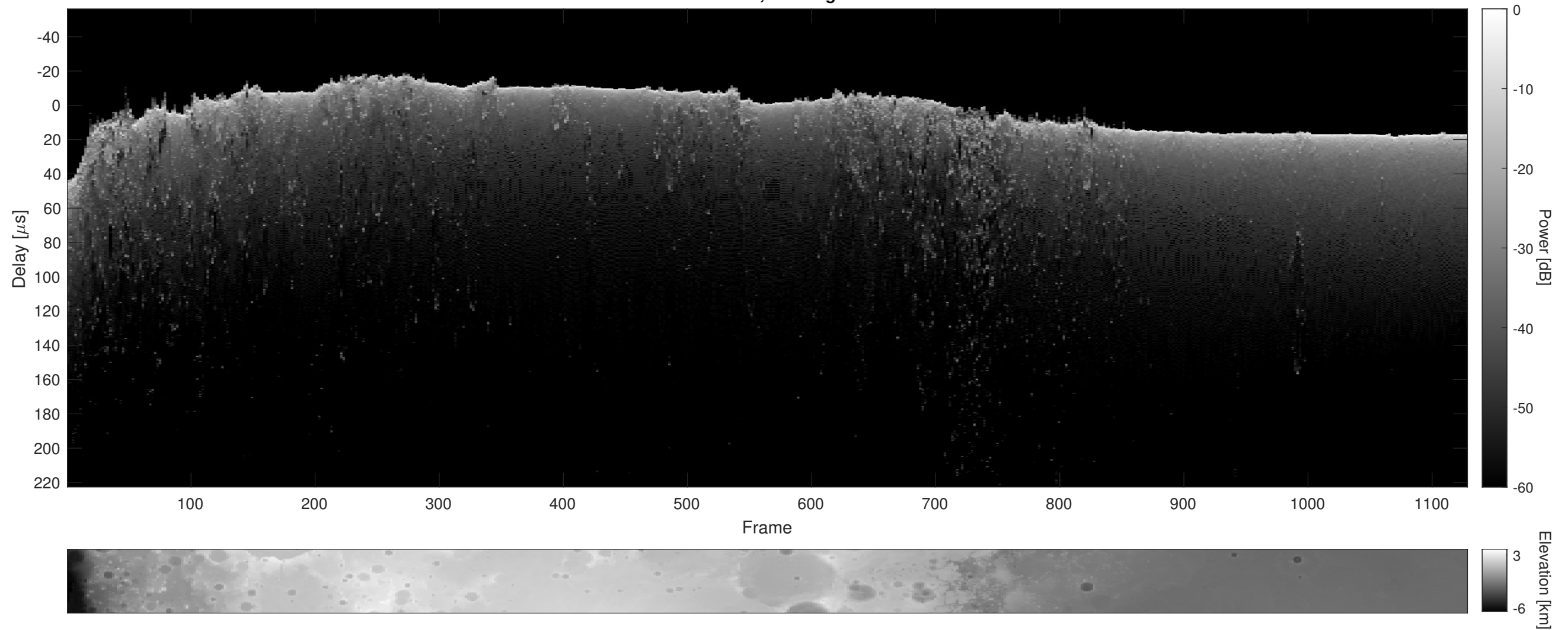
Orbit 14377, Cluttergram
