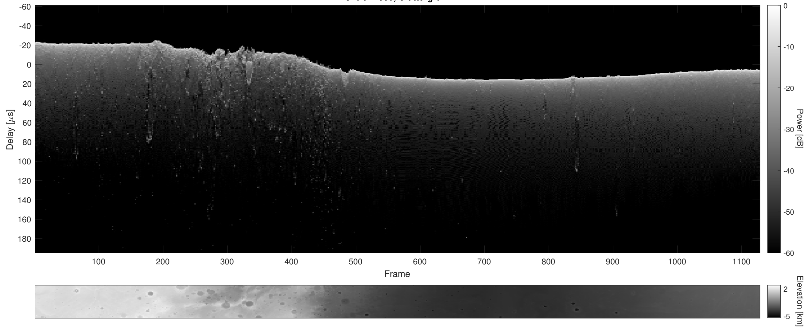
Orbit 14380, Cluttergram
