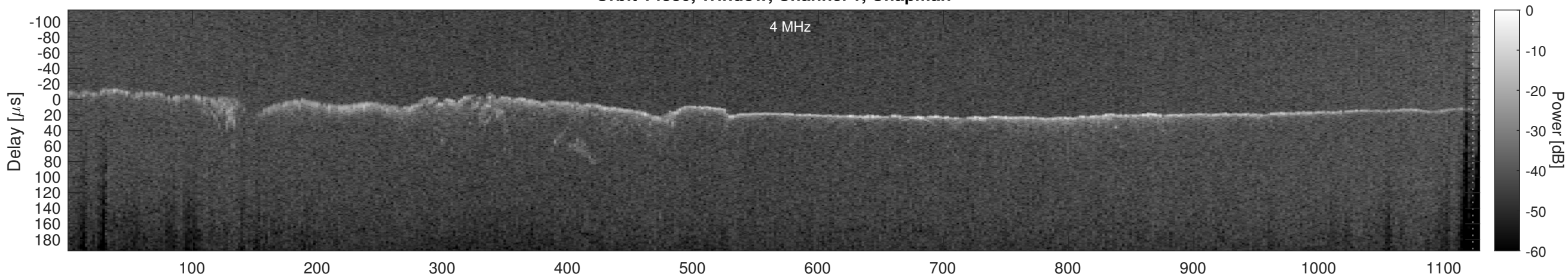
Orbit 14380, Window, Channel 1, Optimized
