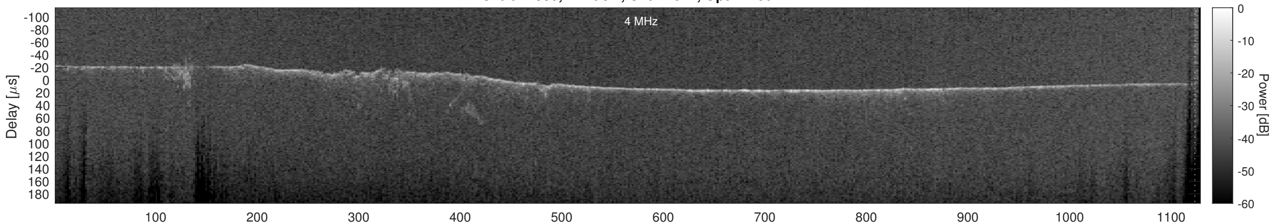
Orbit 14380, Cluttergram
