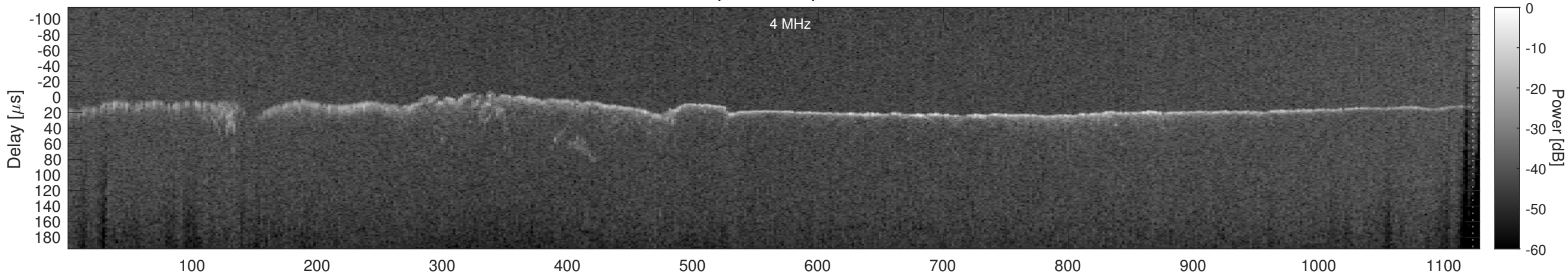
Orbit 14380, Window, Channel 1, Chapman
