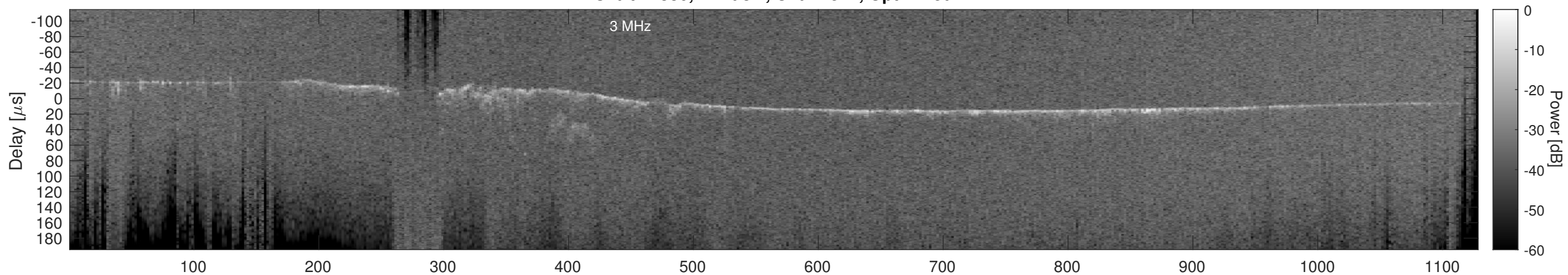
Orbit 14380, Cluttergram
