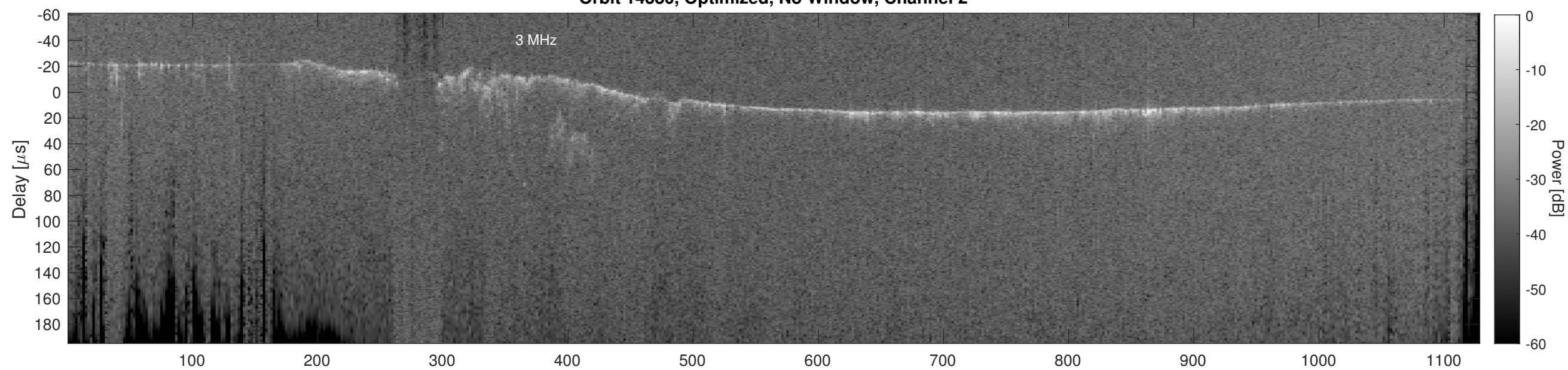
Orbit 14380, Cluttergram
