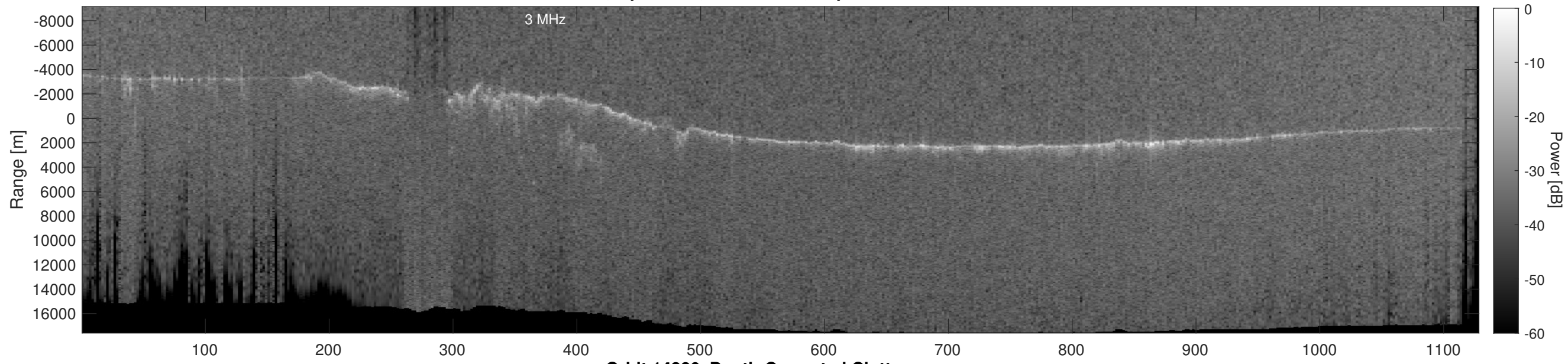
Orbit 14380, Depth-Corrected Cluttergram
