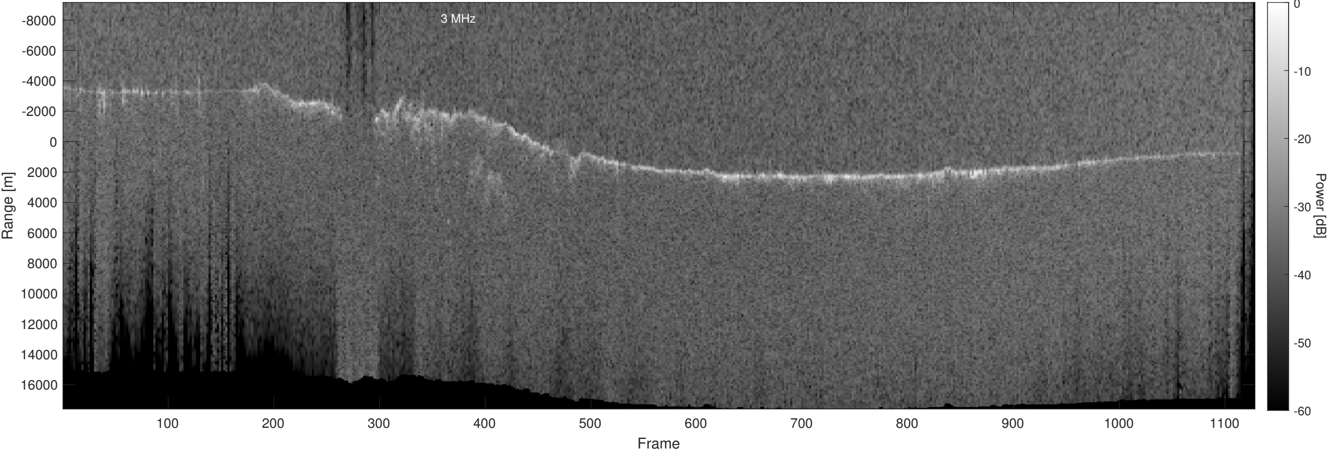
Orbit 14380, Optimized, Window, Depth-Corrected, Channel 2
