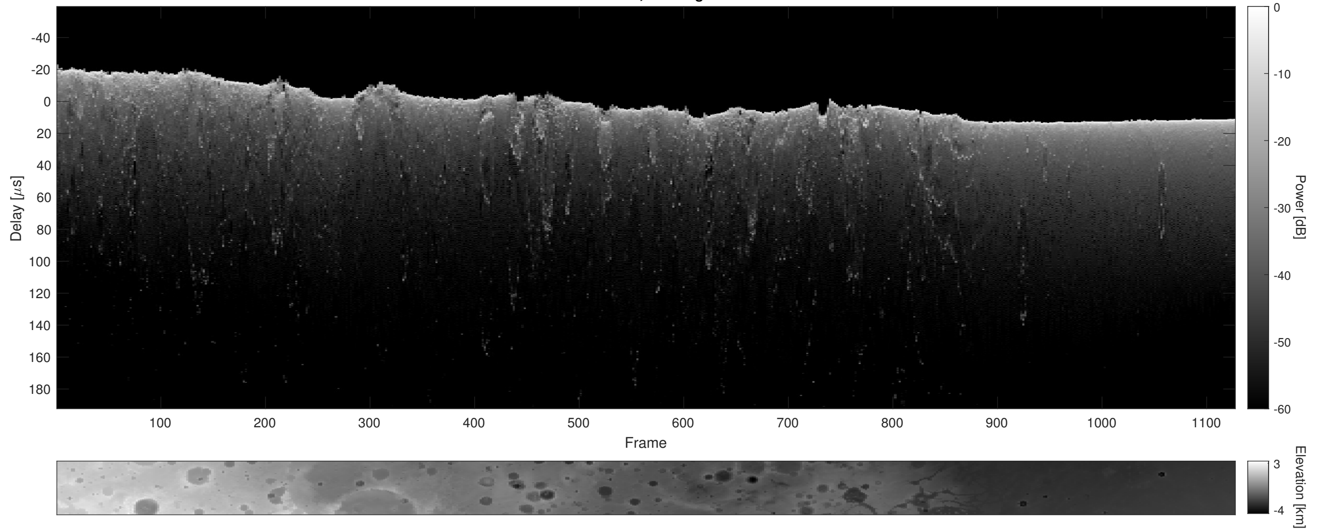
Orbit 14381, Cluttergram
