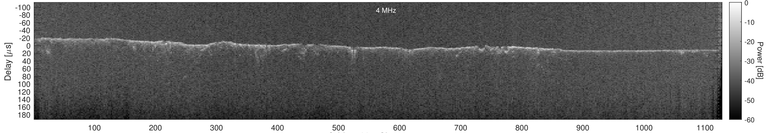
Orbit 14381, Cluttergram
