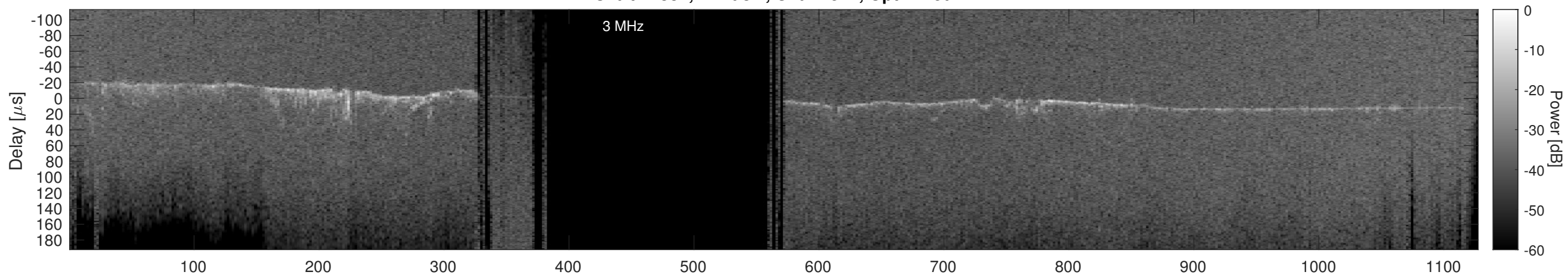
Orbit 14381, Cluttergram
