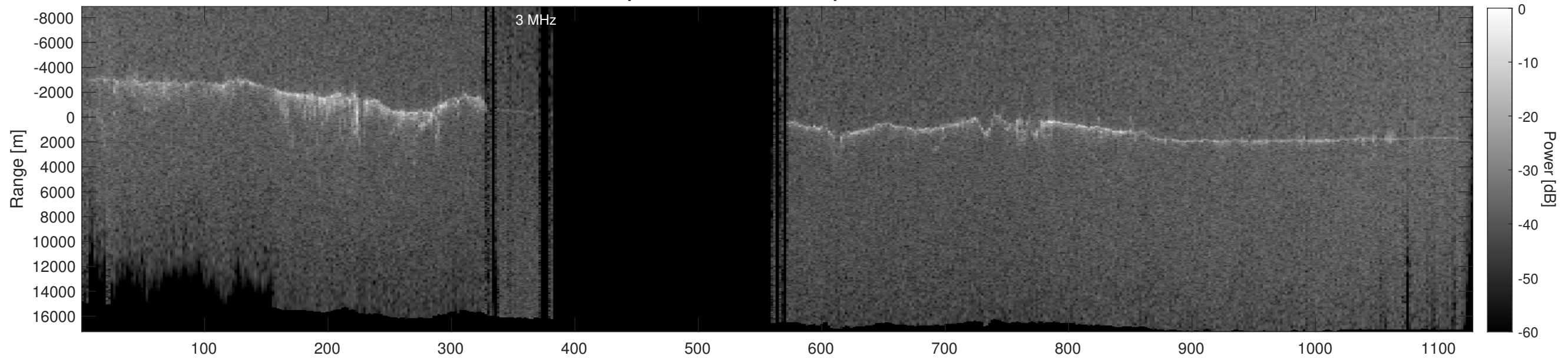
Orbit 14381, Depth-Corrected Cluttergram
