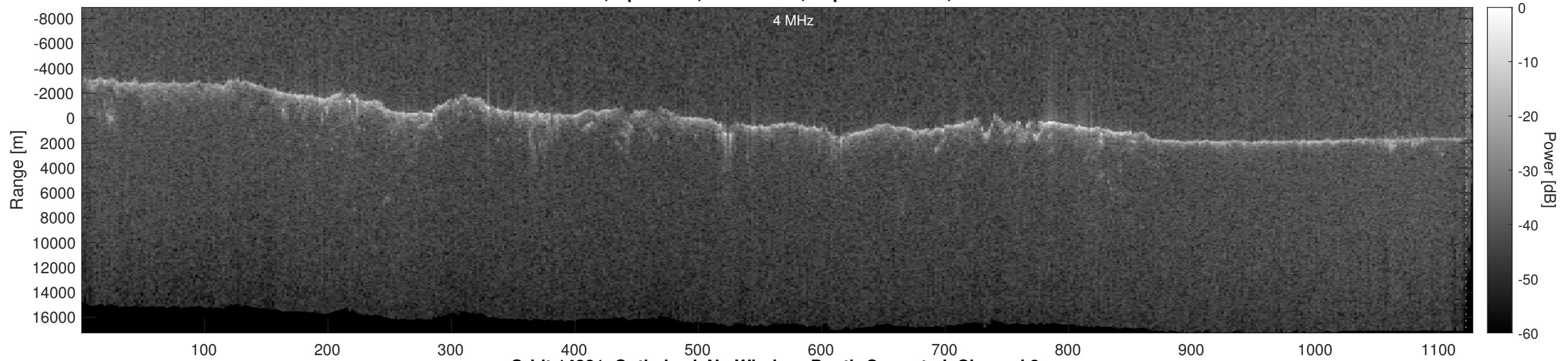
Orbit 14381, Optimized, No Window, Depth-Corrected, Channel 2
