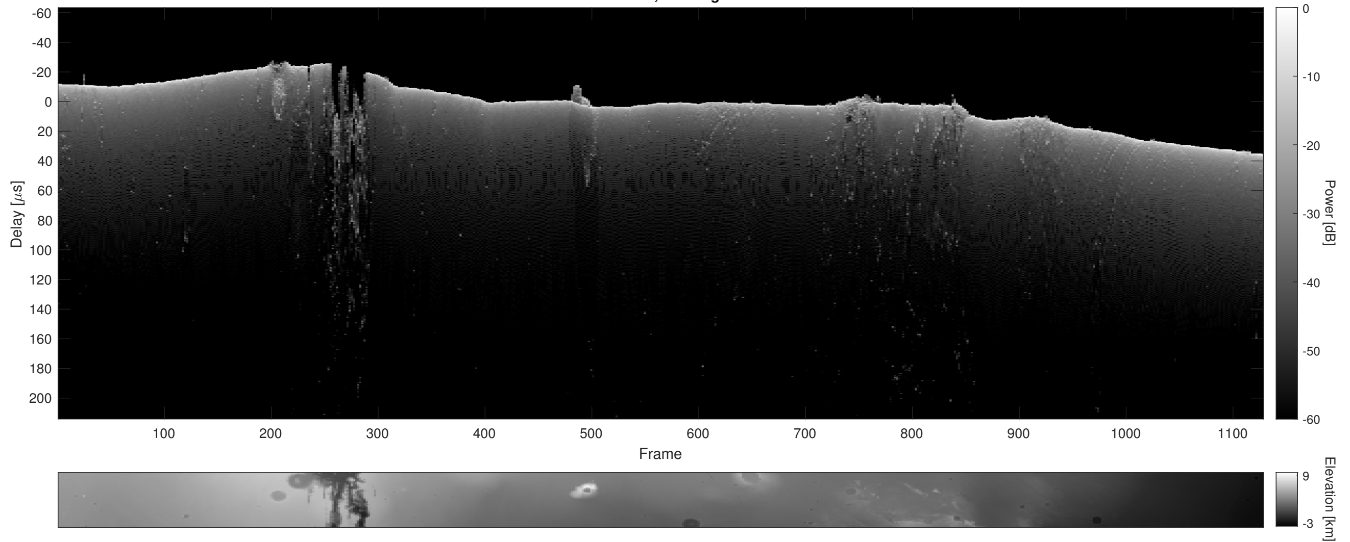
Orbit 14382, Cluttergram
