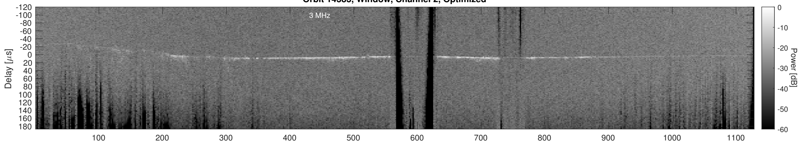
Orbit 14383, Cluttergram
