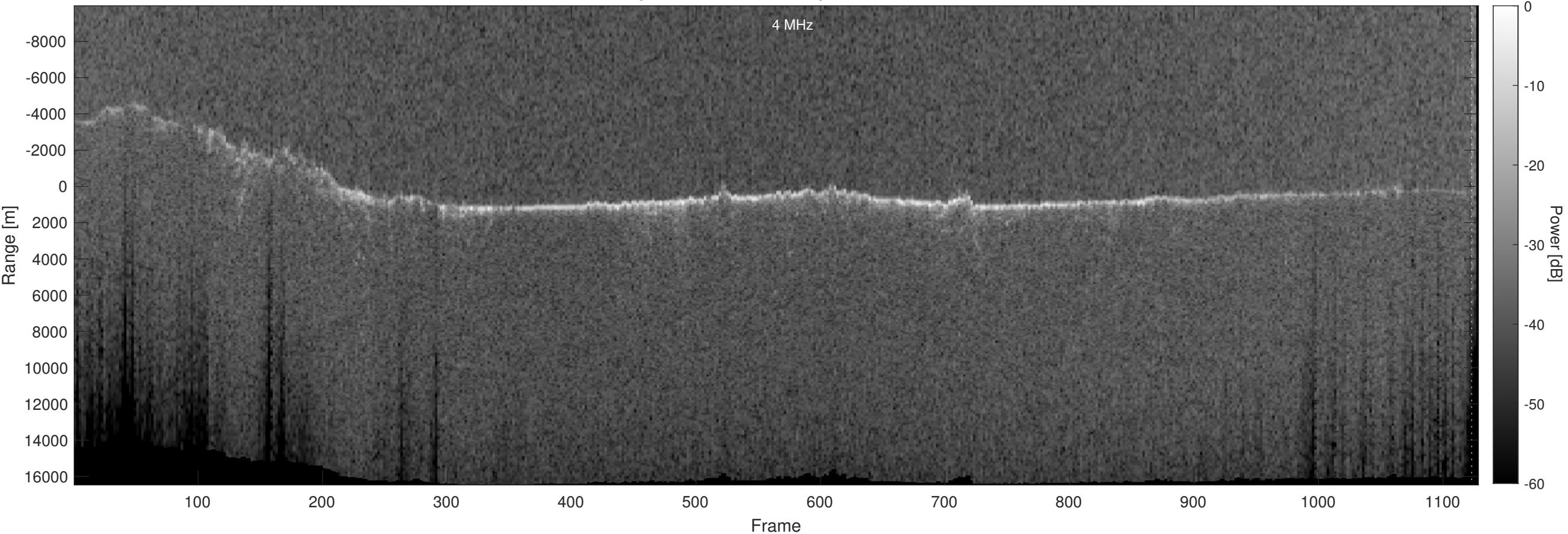
Orbit 14383, Optimized, Window, Depth-Corrected, Channel 2
